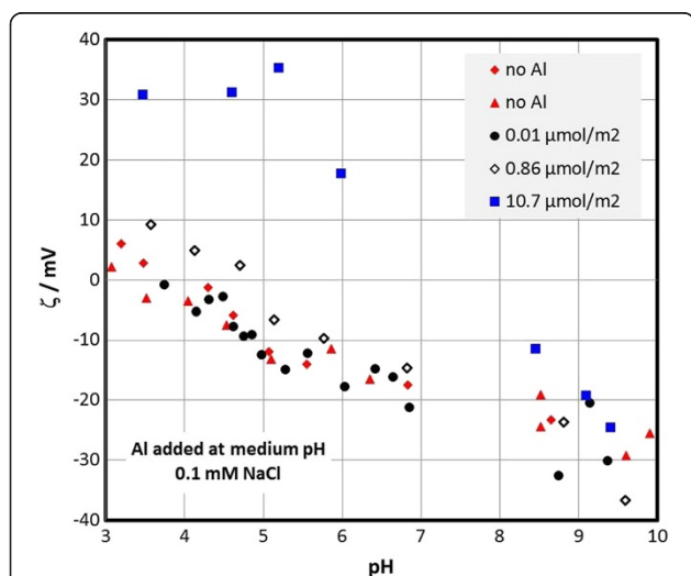
Figure 6 Zeta-potential of kaolinite as a function of pH in 0.1 mM NaCl with and without added aluminum. Total aluminum is given as maximum coverage that could possibly be achieved by the intentionally added aluminum.
