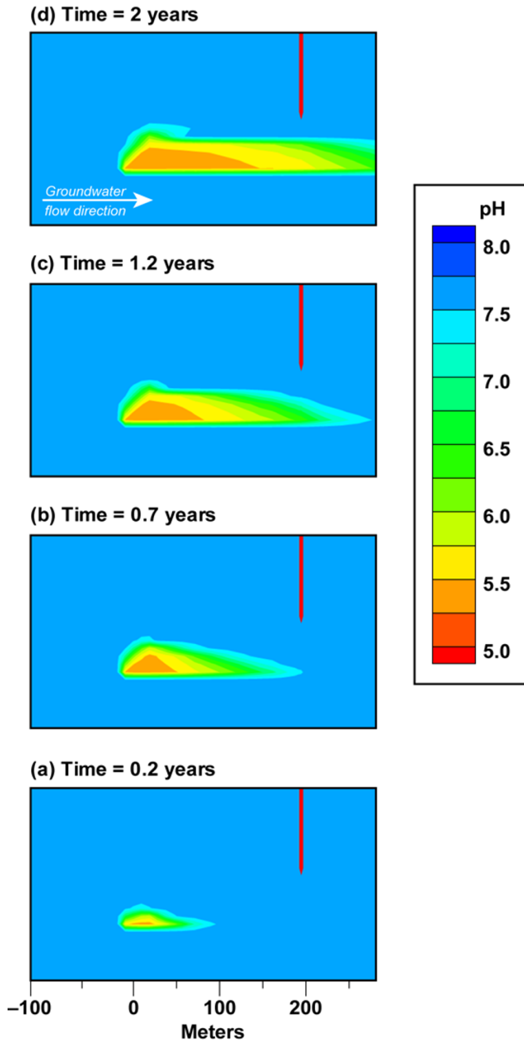
Figure 6 Evolution of pH plume from a CO 2 flux = 10 3 t/yr (0.63 t/m 2 /yr) and 0.3% hydraulic gradient. CO 2 source is at 170 m depth in an aquifer bounded by relatively impermeable clay layers. Plots show plume details between the CO 2 leak source and sampling well at discrete time steps. The full lateral extent of the plume is shown in Movie 2 (see Additional file 2). The plots are also identified on the pH breakthrough curves in Figure 5.
